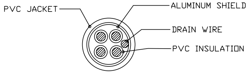
[2464#18AWG 4C+1] SECTIONAL DRAWING
